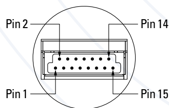
Mating Connector: FI-W15S JAE
